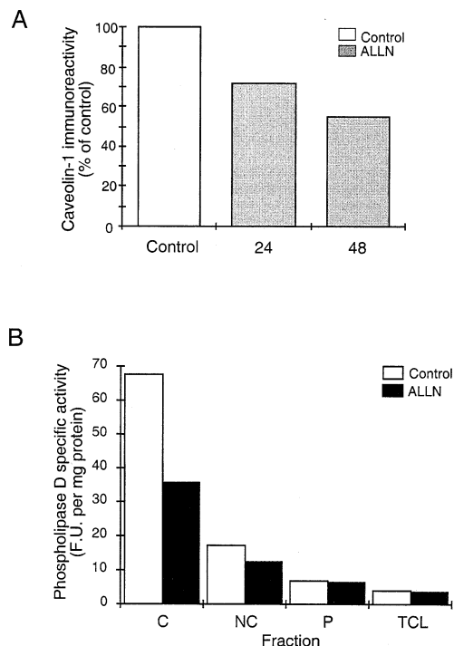
Fig. 5. Effect of ALLN on caveolin-1 expression and PLD activity in HaCaT cells. HaCaT cells were incubated in the absence (control; open bars) or presence of 10 \mu M ALLN (solid bars) for 24 and 48 h as indicated. Cells were harvested in Triton X-100 lysis buffer and subjected to separation on sucrose density gradients as described in Section 2. A: Caveolin-1 immunoreactivity in caveolar fractions (pooled fraction 5, 6 and 7). B: PLD-specific activity in caveolar fractions (C), non-caveolar fractions (NC), insoluble pellet (P) and total cell lysates (TCL) in cells treated for 48 h with 10 \mu M ALLN (black bars).
